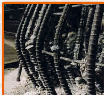
Damage due to insufficient gas pressure welded splices. Longitudinal reinforcement broke at pressure welding portion in Kobe earthquake.
